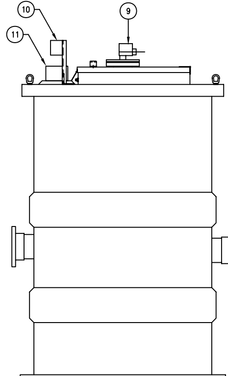
SIDE ELEVATION
