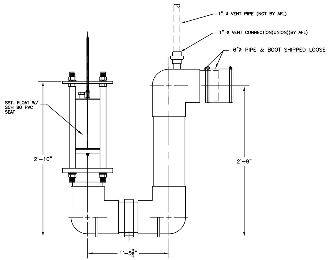
SIDE VIEW
