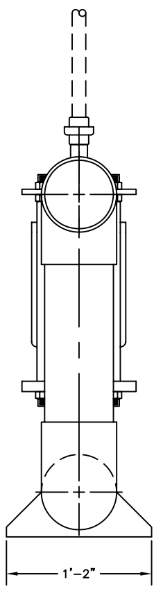
OUTLET VIEW
