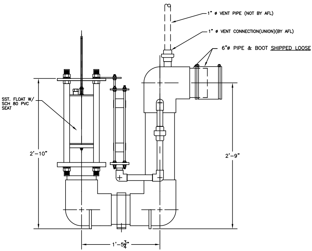
SIDE VIEW
