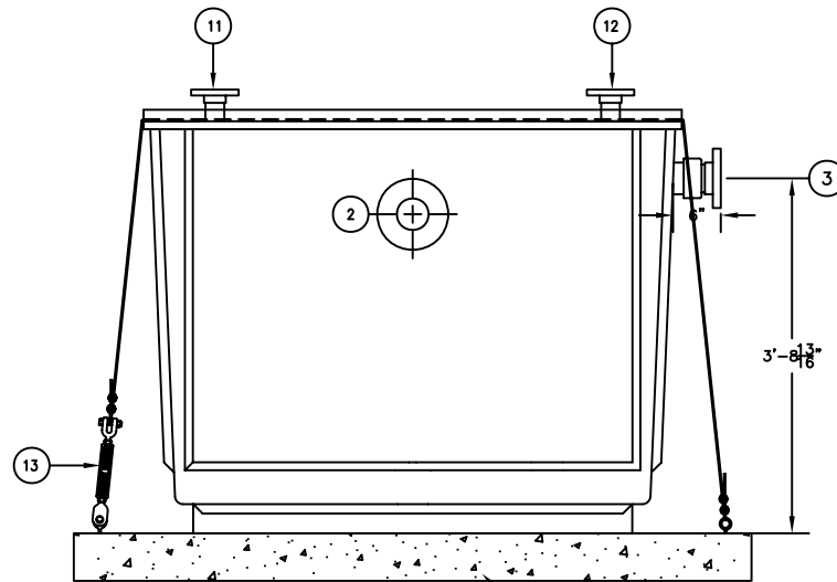
ELEVATION OUTLET END
