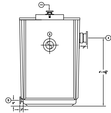
OUTLET END ELEVATION
