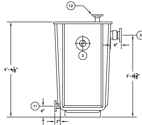
END OUTLET ELEVATION
